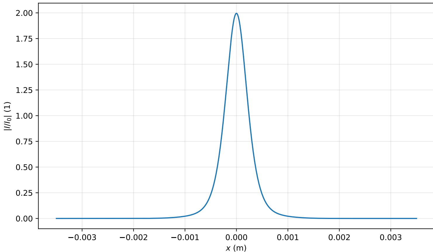
Intensity profile I(x, y = 0, z = 1.751m)/I_0 , P_{in}=1.0P_{cr} , artificial time
